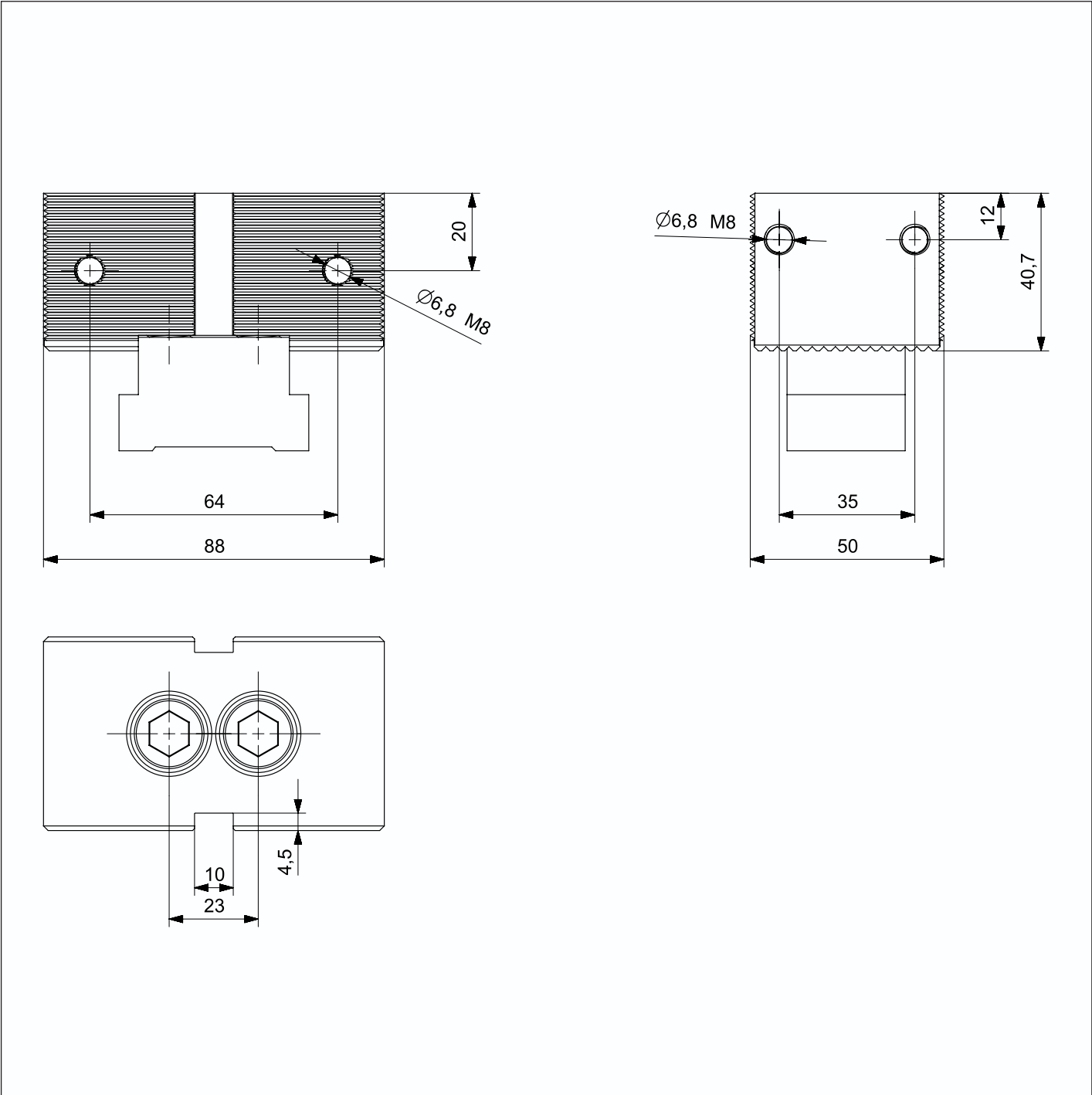
88G-MT 齿型固定钳口 | 88G-MT Serrated stationary wedge
