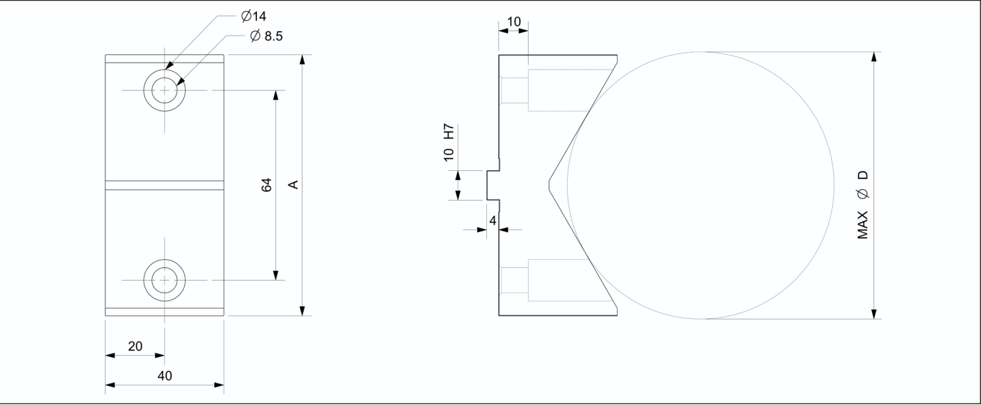
88RZ-V 型软爪 | 88RZ-V type unidirectional clamping jaw
