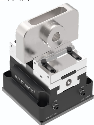
气动自定心虎钳 | Pneumatic self-centering vise
