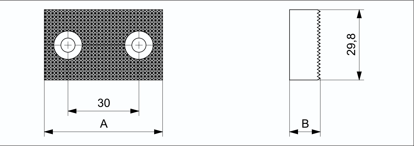
50C 齿型钳口 | 50C Serrated Jaw
