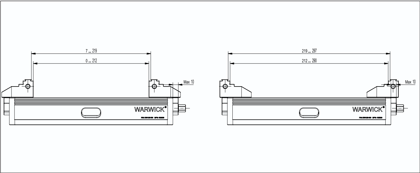
硬爪夹持范围 | Hard jaw clamping range
