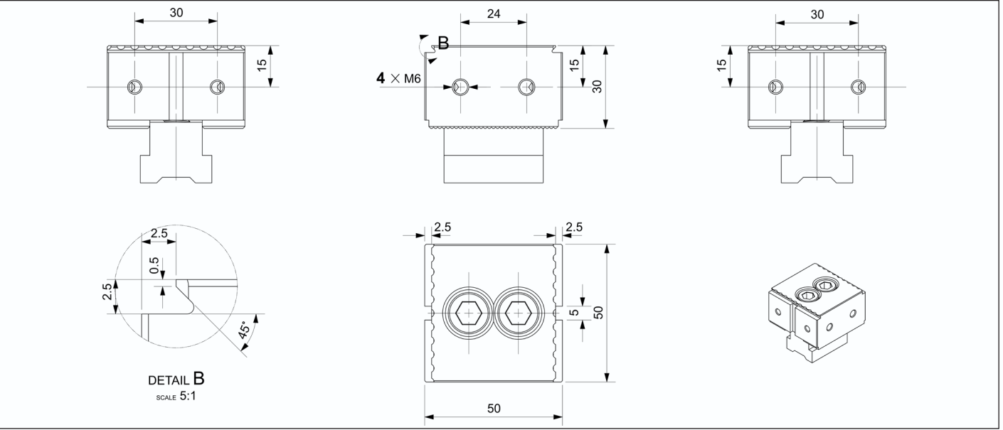
50G-T 锯齿型固定钳口 | 50G-T Serrated Stationary Clamping Jaw
