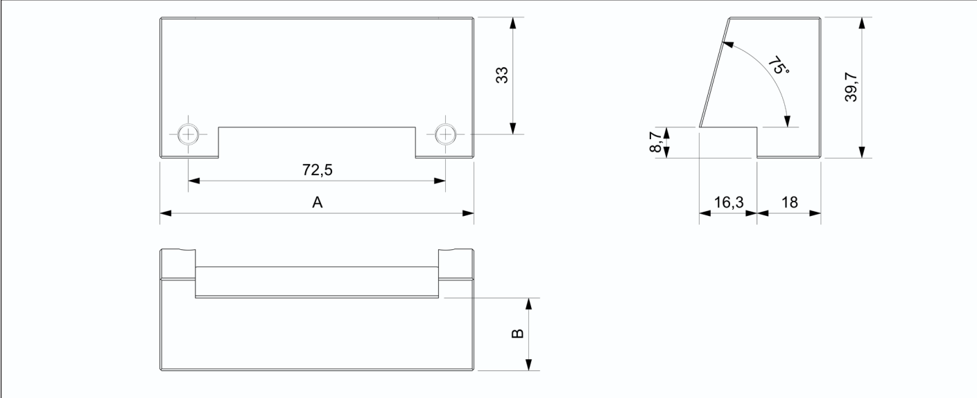
88RZ-C 型软爪 | 88RZ-C type soft jaw
