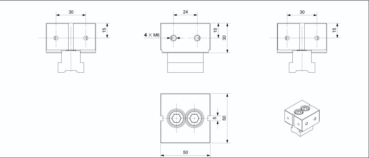
50G 固定钳口 | 50G type Stationary clamping jaw
