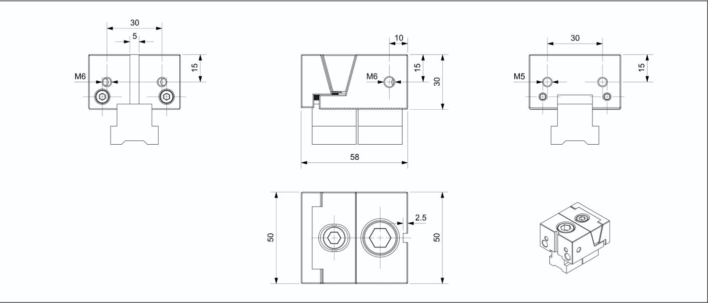
50FD 型单向夹紧钳口 | 50FD type unidirectional clamping jaw
