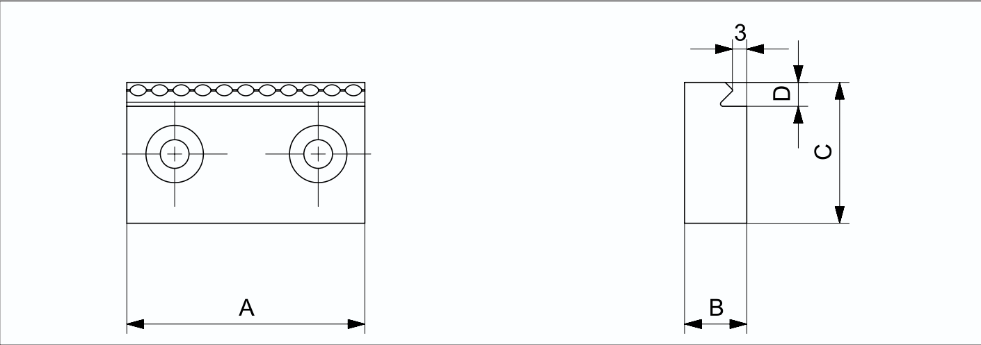
50C-T 齿型台阶钳口 | 50C Serrated Step Jaw
