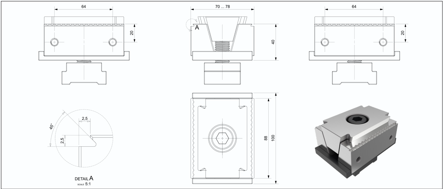
88MD-T 锯齿型双向夹紧钳口 | 88MD-T Jagged type Bidirectional Clamping Jaw
