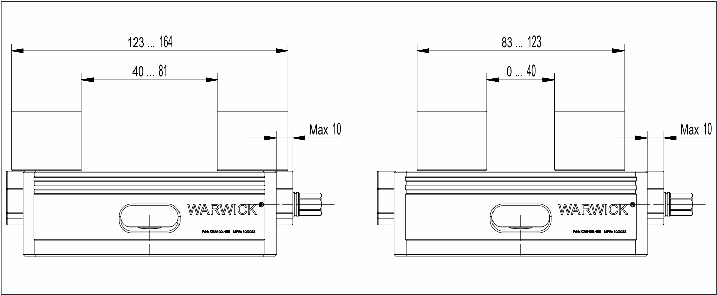
软爪夹持范围 | Soft jaw clamping range
