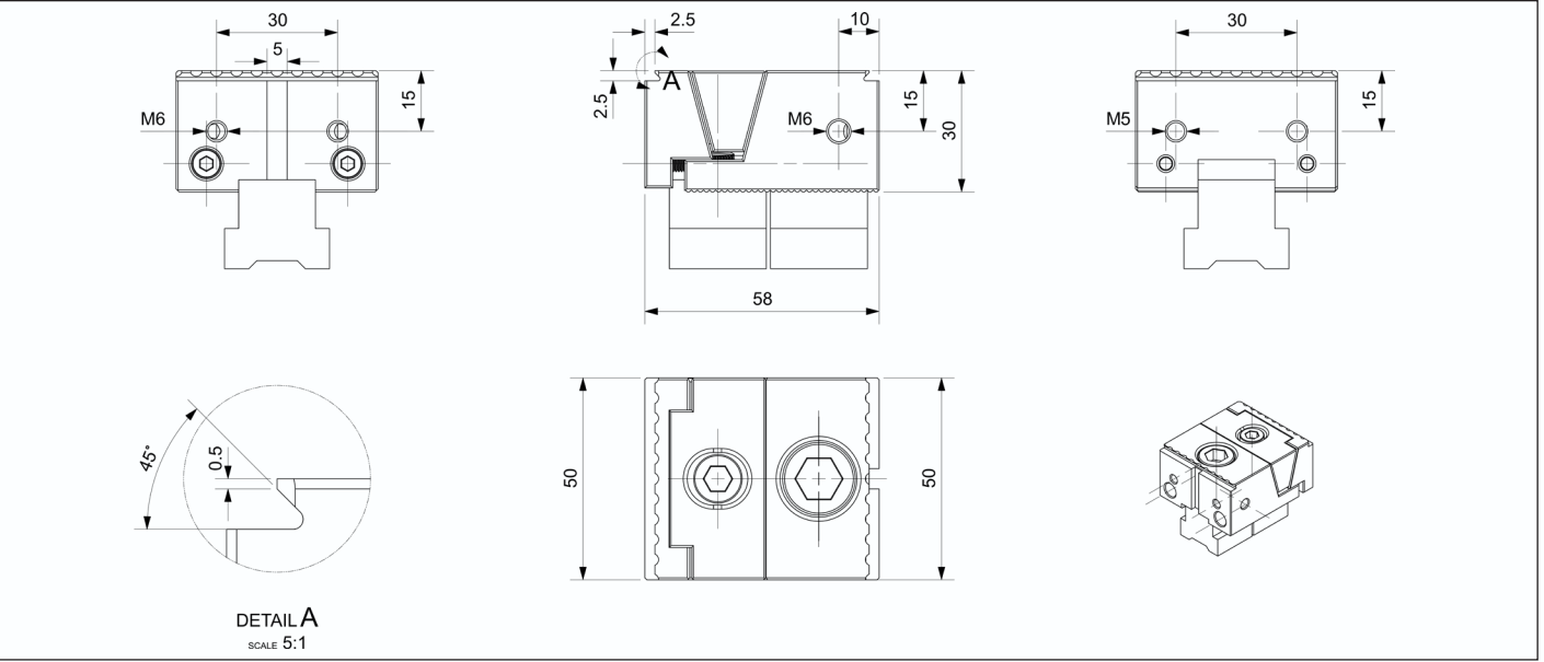
50FD-T 锯齿形型单向夹紧钳口 | 50FD-T Jagged type unidirectional clamping jaw
