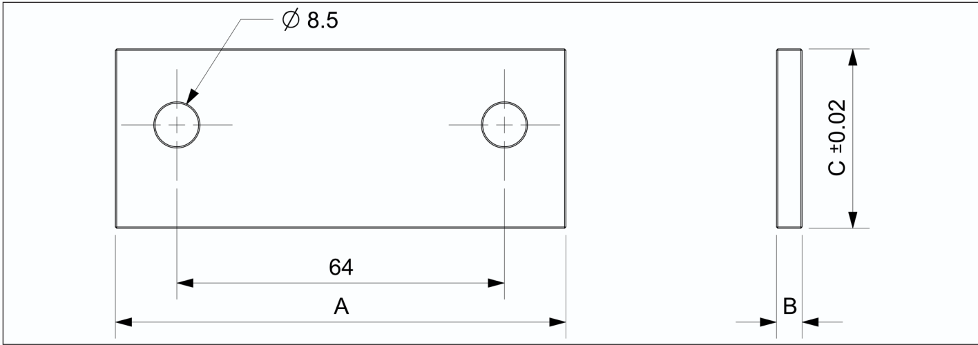
88DP 平行垫块 | 88DP Parallel gasket
