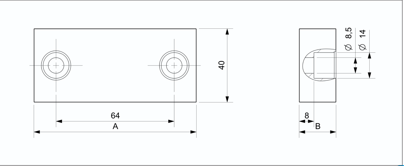
88RZ-B 型软爪 | 88RZ-B type soft jaw
