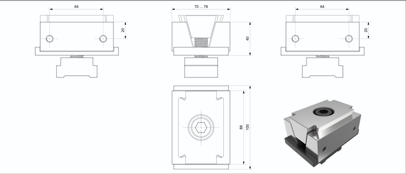
88MD 型双向夹紧钳口 | 88MD type Bidirectional Clamping Jaw
