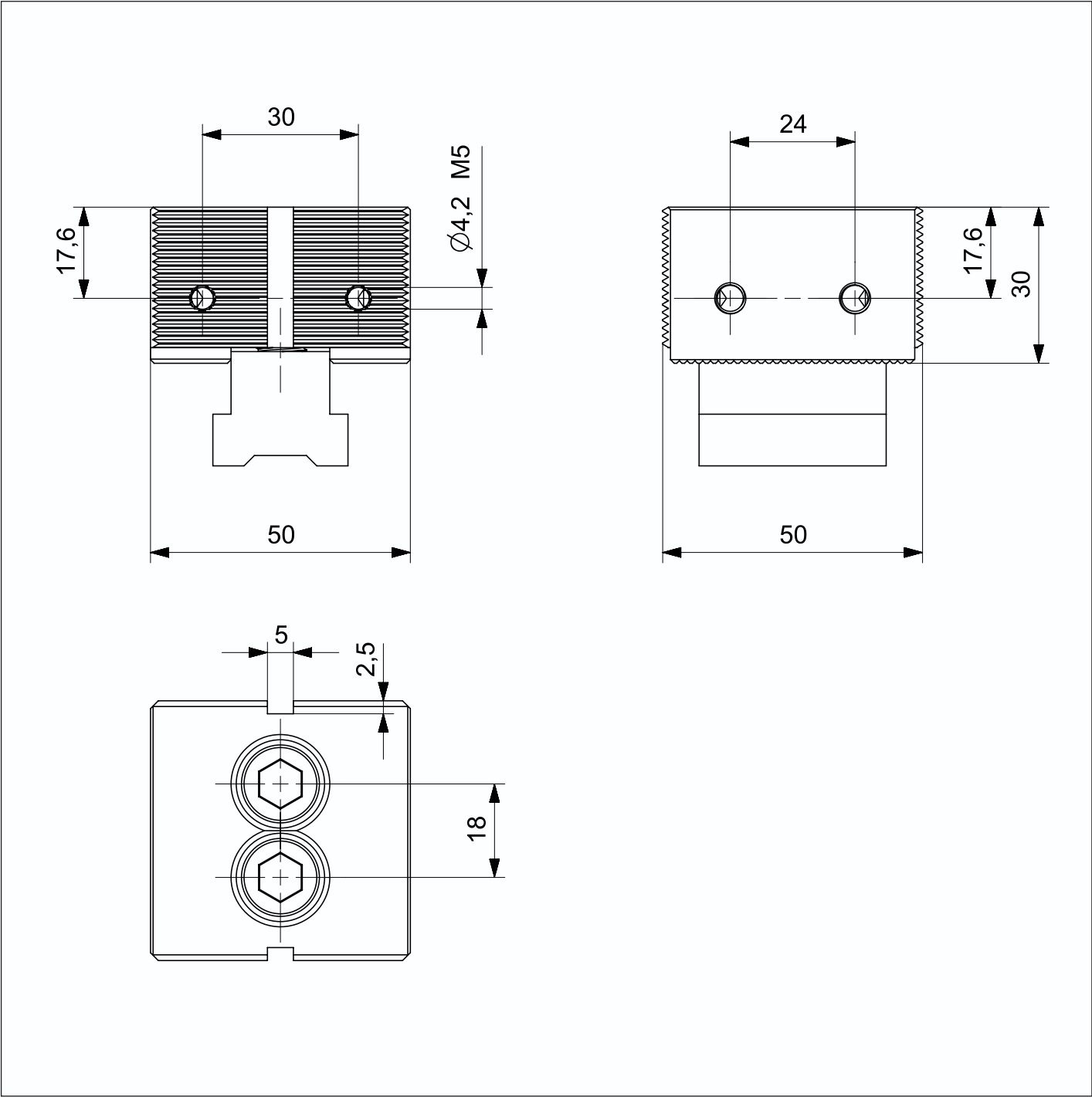
50G-MT 齿型固定钳口 | 50G-MT serrated fixed Jaw
