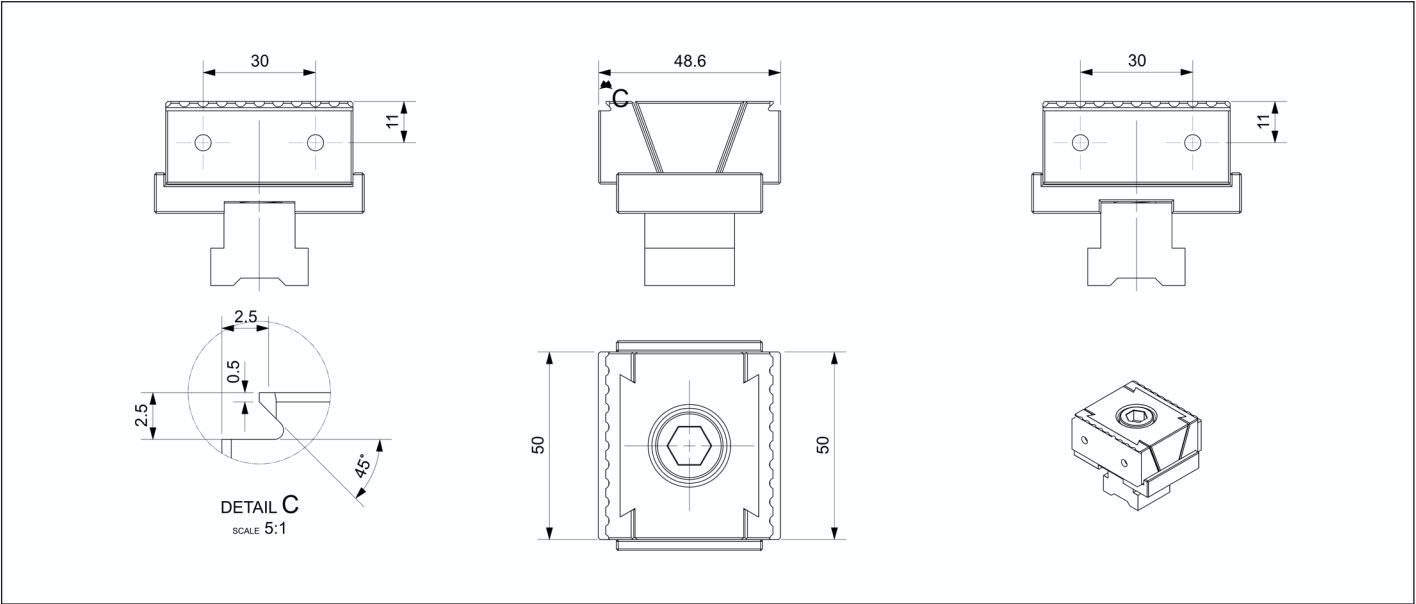
50MD-T 锯齿型双向夹紧钳口 | 50MD-T Jagged type Bidirectional Clamping Jaw
