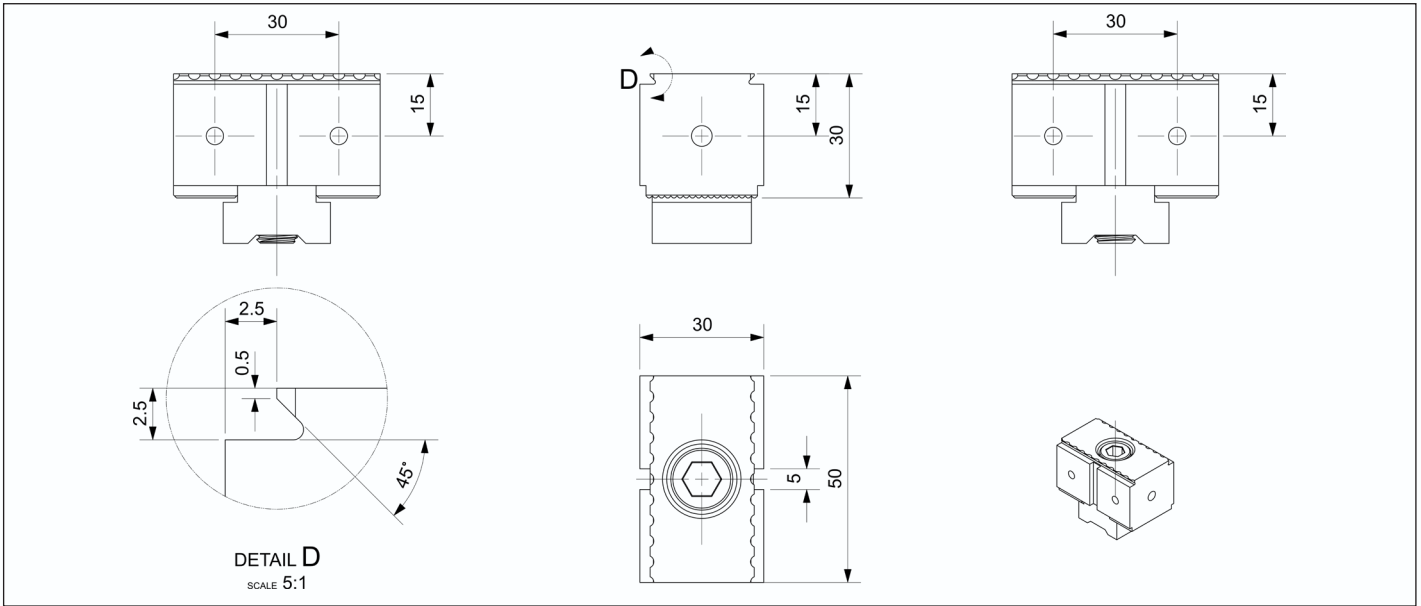
50SG-T 锯齿型固定钳口 | 50SG-T Serrated fixed jaw
